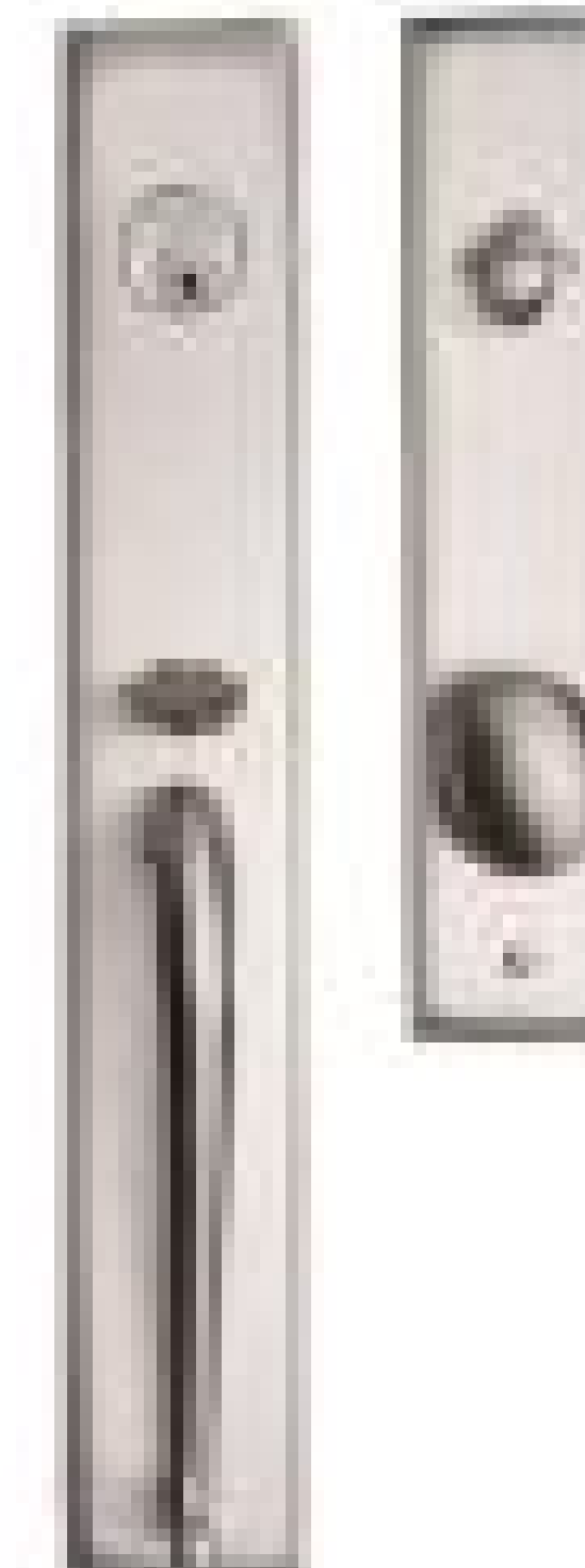
SQTUB Escutcheon Exterior: 18" x 3" Interior: 11" x 2 1/2" Windsor 9000 knob in Satin Nickel
