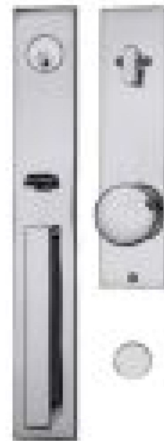
UBTUB Escutcheon Exterior: 17" x 2 1/2" Interior: 10 1/2" x 2 1/2" Helios 8800 knob in Polished Chrome
