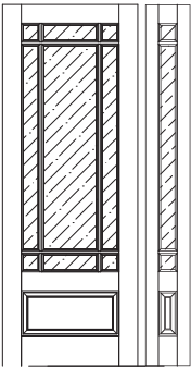
GP910 Door and Sidelite
