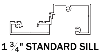
1 3/4" STANDARD SILL
