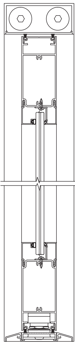
HEAD & SILL DETAILS
