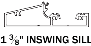
1 3/8" INSWING SILL
